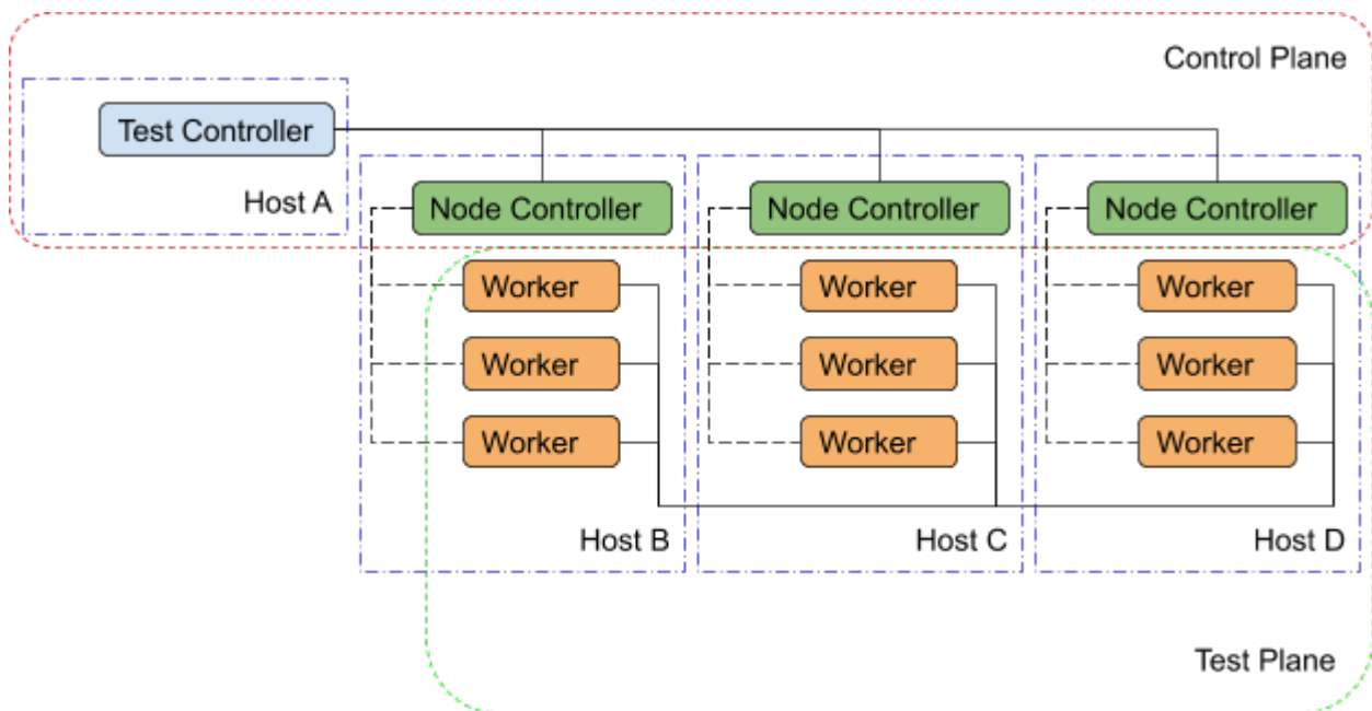
Fig. 1: Bench Overview
